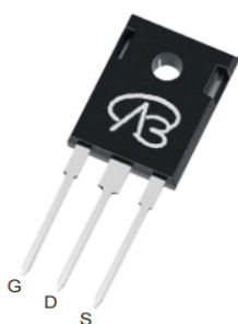
TO-247
