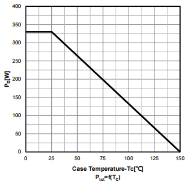
Power dissipation
