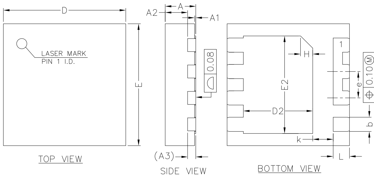
DFN3x3
