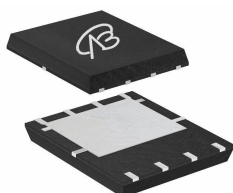
DFN3x3
