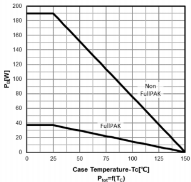
Power dissipation
